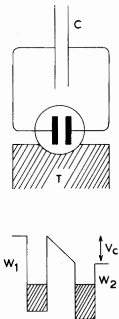
Fig. 16. Alkemade's diode.
