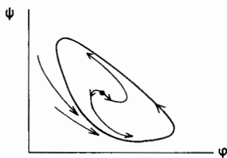
Fig. 43. Limit cycle surrounding an unstable point.
