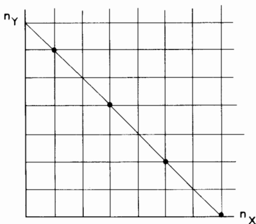
Fig. 18. Accessible states for 2X \rightleftharpoons 2Y with A = 7 .
