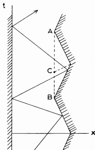
Fig. 12. Hammersley's model of a bouncing particle.
