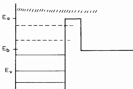
Fig. 20. Bound states, approximately bound states and decaying states.
