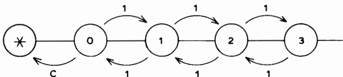
Fig. 14. Random walk with absorbing boundary.
