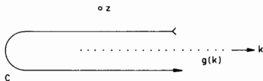
Fig. 48. The poles k_n and the contour C .
