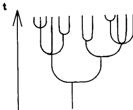
Fig. 3. One realization of a general branching process.
