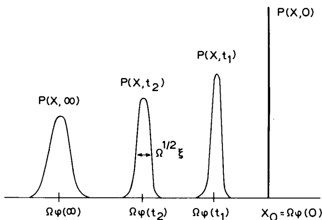
Fig. 23. The evolution of the probability density.
