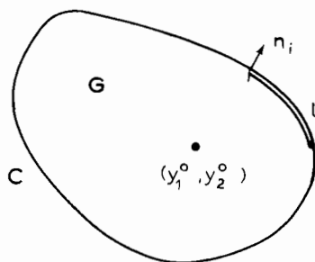
Fig. 32. The region G enclosed by the curve C with arc length l and normal n .
