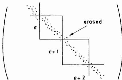
Fig. 50. The operator A in the representation of H .
