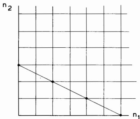
Fig. 19. The state space for the dissociation reaction (3.5) with n_2^0 = 3 .
