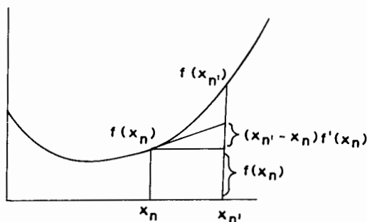
Fig. 10. A property of convex functions.
