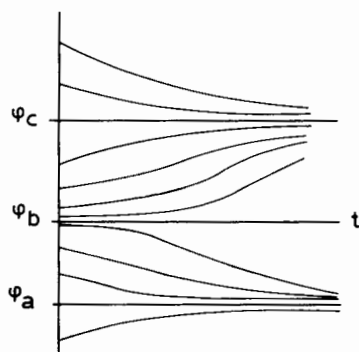
Fig. 28. All solutions other than \phi_b itself tend to either \phi_a or \phi_c .
