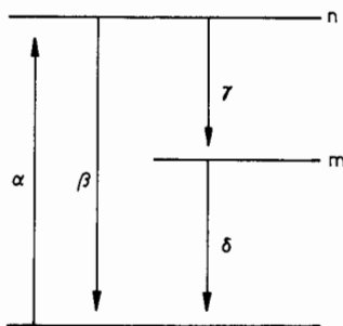
Fig. 45. The transitions in the three-level atom.
