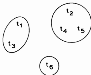
Fig. 2. The term (5.2) in the cluster expansion of f_6 .
