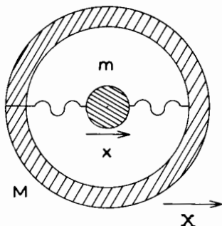
Fig. 22. Simplified itinerant oscillator model.
