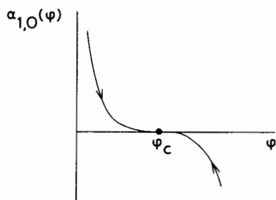
Fig. 39a. The critical point.
