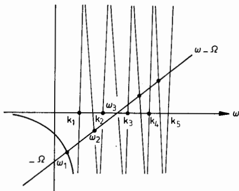
Fig. 47. Graphical solution of (2.8).
