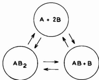
Fig. 9. An example of detailed balance.
