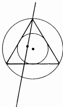
Fig. 1. Bertrand's circle with random chord.
