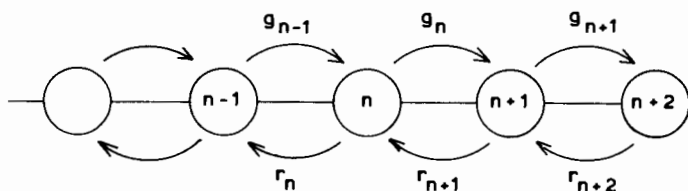
Fig. 11. The one-step process and its transition probabilities.
