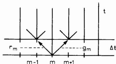
Fig. 33. The derivation of the equations for \pi_m , \tau_m , g_m .
