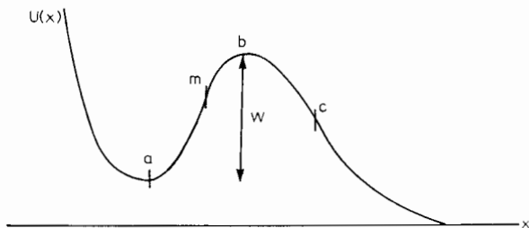
Fig. 40. Kramers' potential for a chemical reaction.
