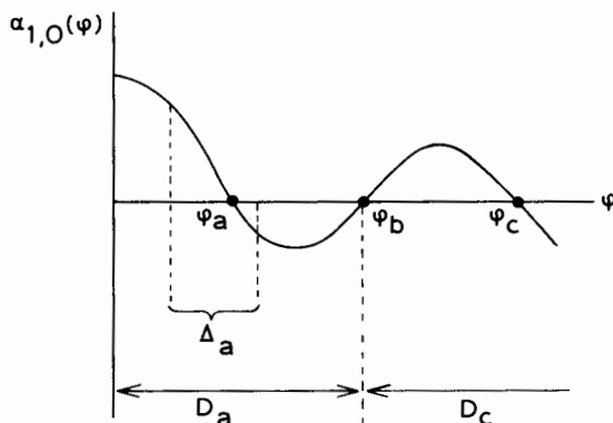
Fig. 34. The macroscopic rate equation for a bistable system and the domains of attraction.
