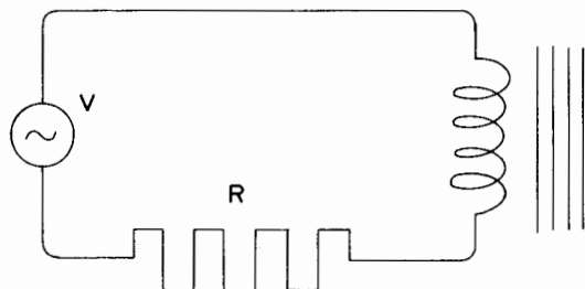
Fig. 46. Nonlinear circuit with random potential generator.
