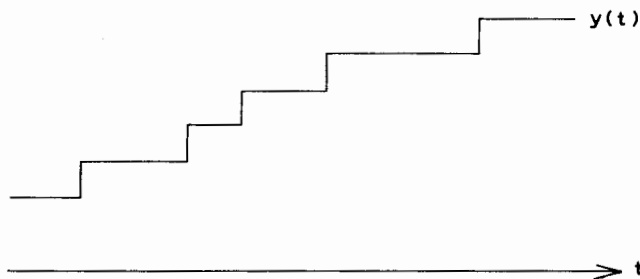
Fig. 5. A sample function of the Poisson process.
