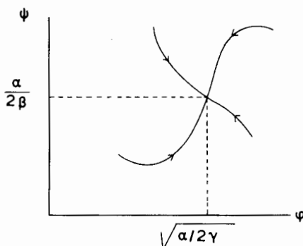
Fig. 29. Solution curves of (5.5).
