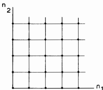
Fig. 17. The state space of a binary mixture.
