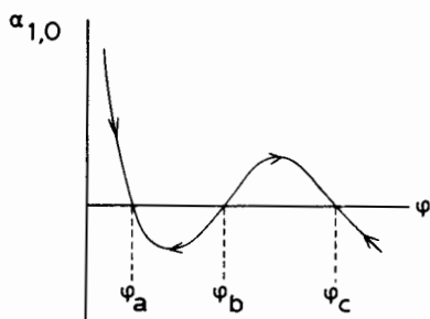
Fig. 27. Two locally stable stationary solutions separated by an unstable one.
