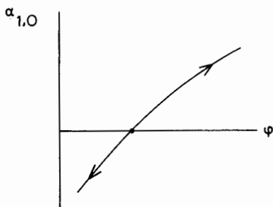
Fig. 24b. Unstable stationary solution.
