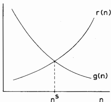
Fig. 21. The stationary state as a balance between generation and recombination.
