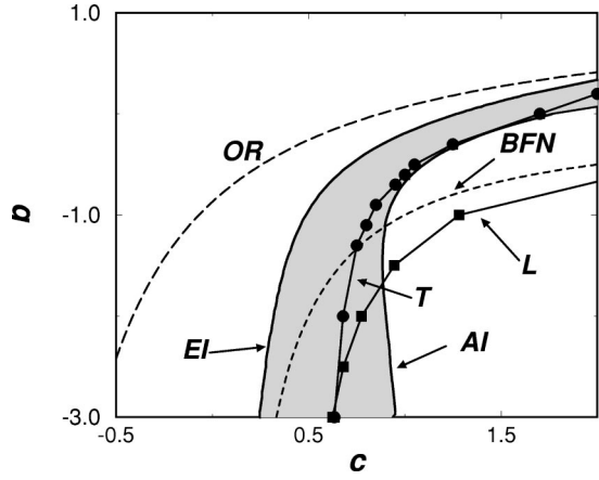
FIG. 12. Stability limits of a spiral wave solution. The boundary of convective (EI) and absolute instability (AI) for the waves emitted by the spiral are also shown (for an explanation see Sec. II.E and Aranson et al. , 1992). Bound states exist to the right of the OR line (c-b)/(1+bc)=0.845 . BFN indicates the Benjamin-Feir-Newell limit 1+bc , L shows the limit of 2D phase turbulence, and line T corresponds to the transition to defect turbulence for random initial conditions. From Chaté and Manneville (1996).
