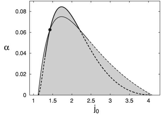
FIG. 1. Bifurcation lines for the Turing (thick line) and the Hopf instability (thin line) in the j_0 - \alpha parameter plane for D=5 and T=0.05 . Broken/solid lines indicate that the bifurcation is sub/supercritical (cf. Sec. III). Grayshading marks the region where the trivial fixed point is unstable. The lefthand Turing-Hopf point is indicated.
