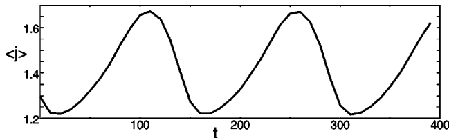
FIG. 6. Time dependence of the spatial average of the current density for the state displayed in Fig. 5.
