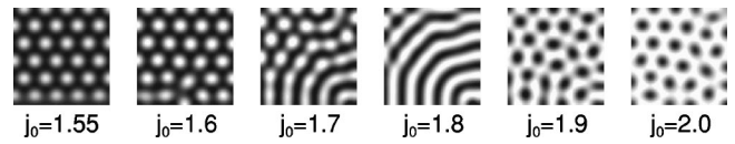
FIG. 8. Time independent patterns appearing for different values of the total current j_0 at \alpha=0.075 , T=0.05 , and D=5 : Transition from hot spots (left) to cold spots (right). Simulations have been performed on a system of size 200 \times 200 with Neumann boundary conditions.
