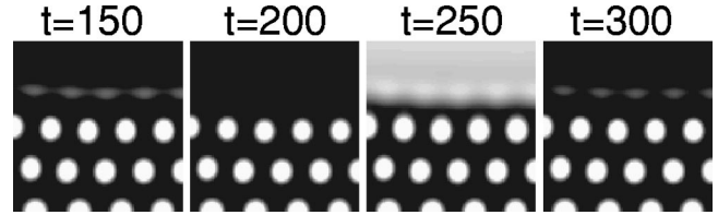
FIG. 5. Coexistence pattern between Turing and Hopf state at j_0 = 1.43 and \alpha = 0.045 . The density plots show the current density j(\mathbf{r}, t) at four different times. The time labels refer to Fig. 6.
